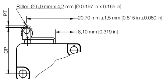
Figure 23. V15 Series A05/Short Roller Lever
