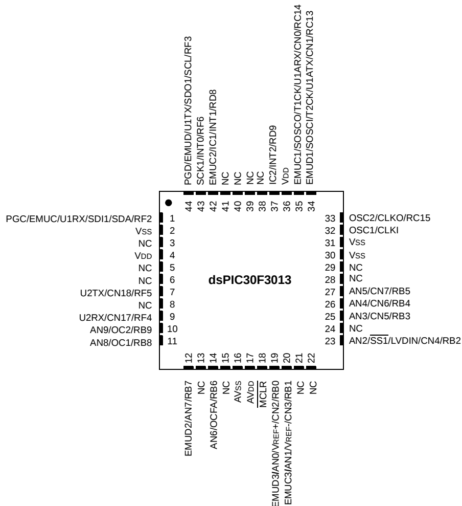
44-Pin QFN (1)
