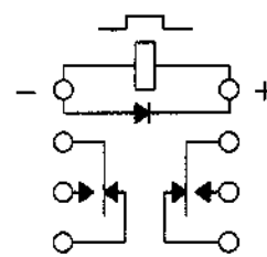
TERMINAL VIEW
