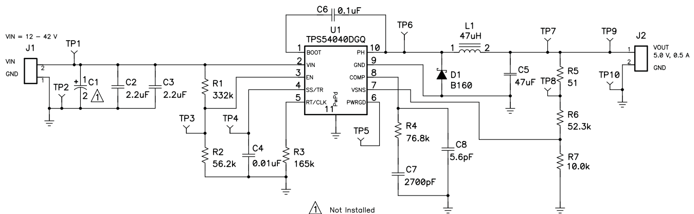
Figure 14. TPS54040EVM-456 Schematic
