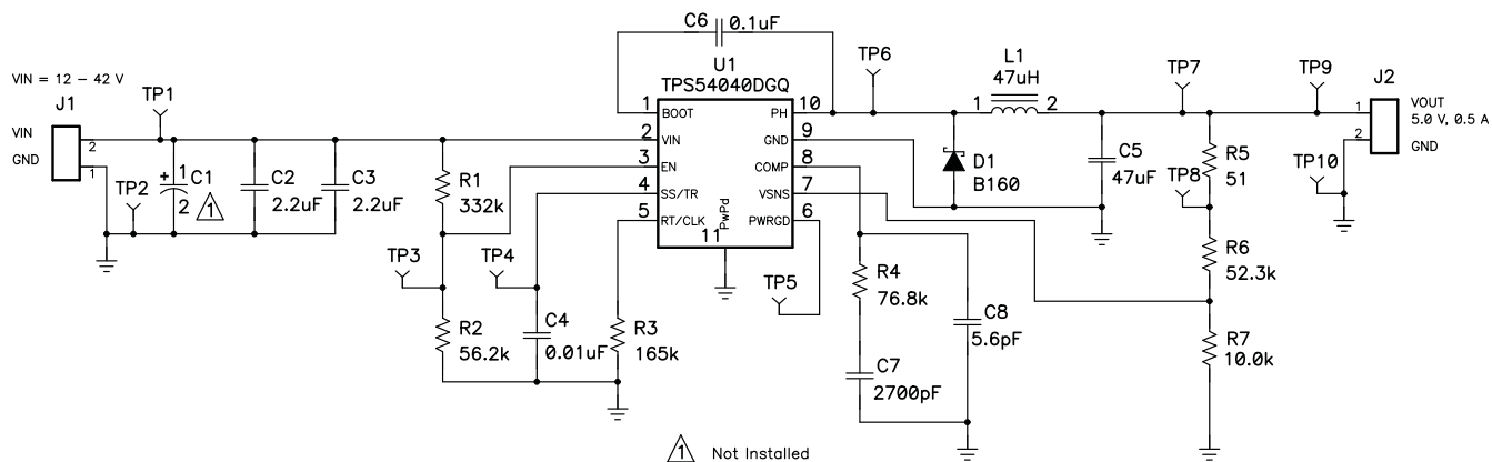
Figure 14. TPS54040EVM-456 Schematic
