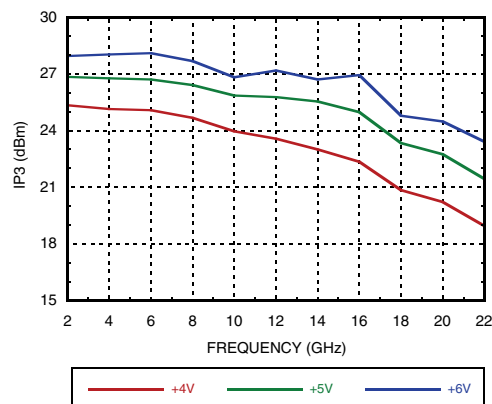
Output IP3 vs. Vdd @ Pout = 4 dBm Tone
