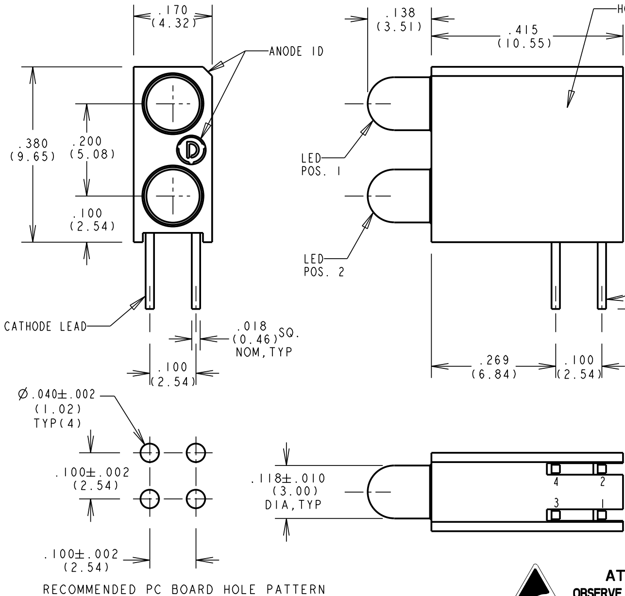
RECOMMENDED PC BOARD HOLE PATTERN
