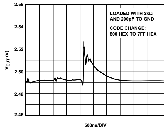
Figure 22. Digital-to-Analog Glitch Impulse
