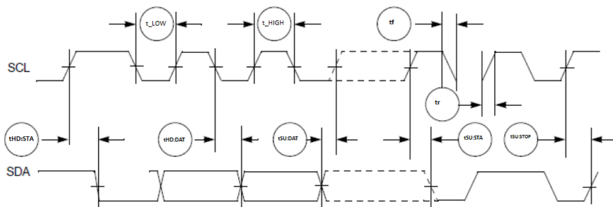
Figure 17. I²C input/output timing
