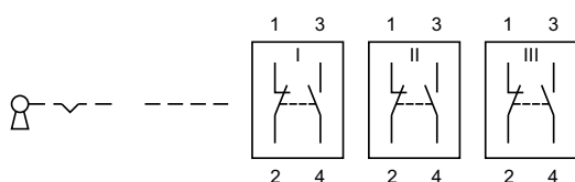
46 Keylock switch 2 positions page 11 | Keylock switch actuator 2 positions, flush mounting page 15
