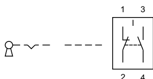
44 Keylock switch 2 positions page 11 | Keylock switch actuator 2 positions, flush mounting page 15
