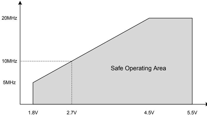
Figure 33-1. Maximum Frequency vs. V_{DD} for [-40, 105]^{\circ}\text{C}
