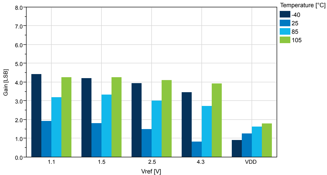
Figure 34-46. Gain Error vs. V_{ref} ( V_{DD}=5.0\text{V} , 115kps)
