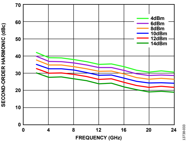
Figure 33. Second-Order Harmonic vs. Frequency for Various P_{OUT} Values, V_{DD} = 10\text{ V} , V_{GG} = 3.5\text{ V} , and I_{DD} = 175\text{ mA}
