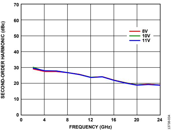
Figure 34. Second-Order Harmonic vs. Frequency for Various V_{DD} Values at P_{OUT} = 14\text{ dBm} and I_{DD} = 175\text{ mA}
