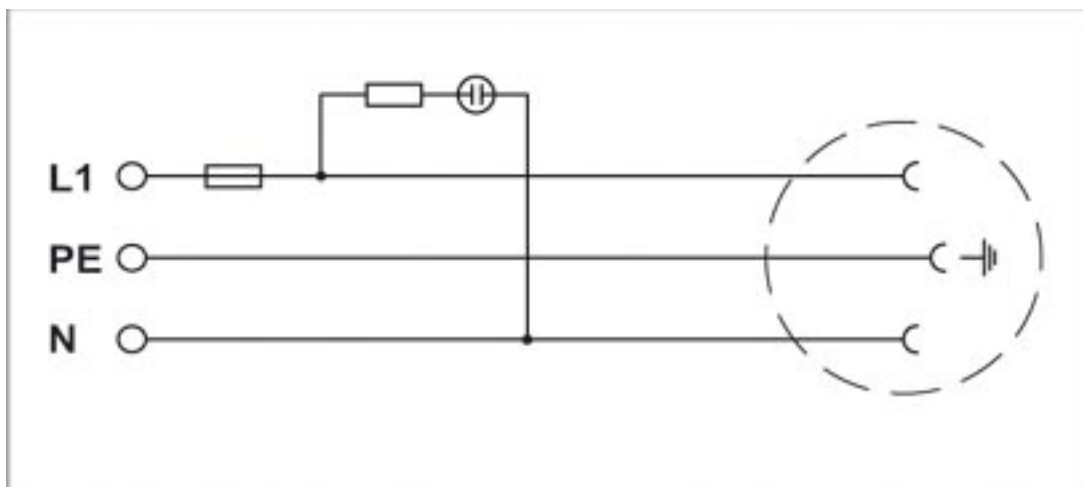
Circuit diagram
