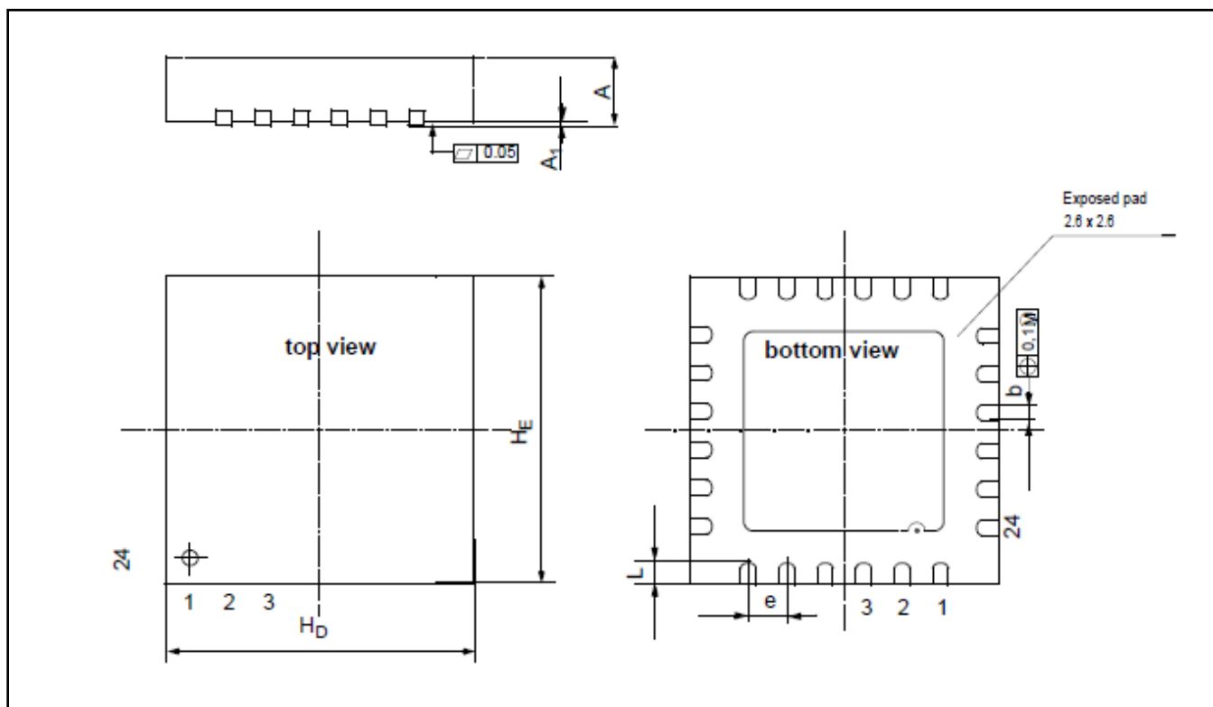
Figure 6.1 Package Drawing
