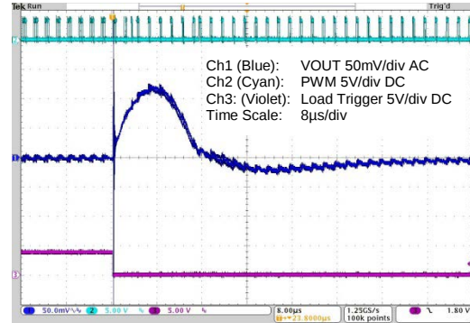
Figure 5.10 VOUT Range #1 with Capacitor Range #2 – Load Step 15 to 5A, Min. Capacitance
