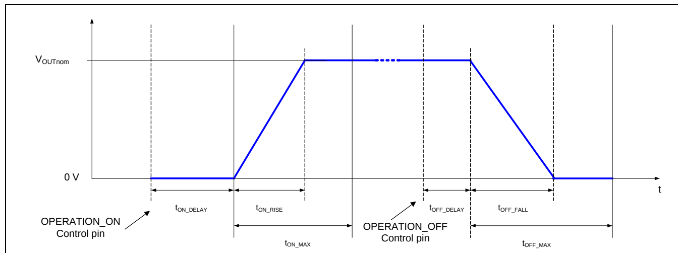
Figure 3.2 Power Sequencing
