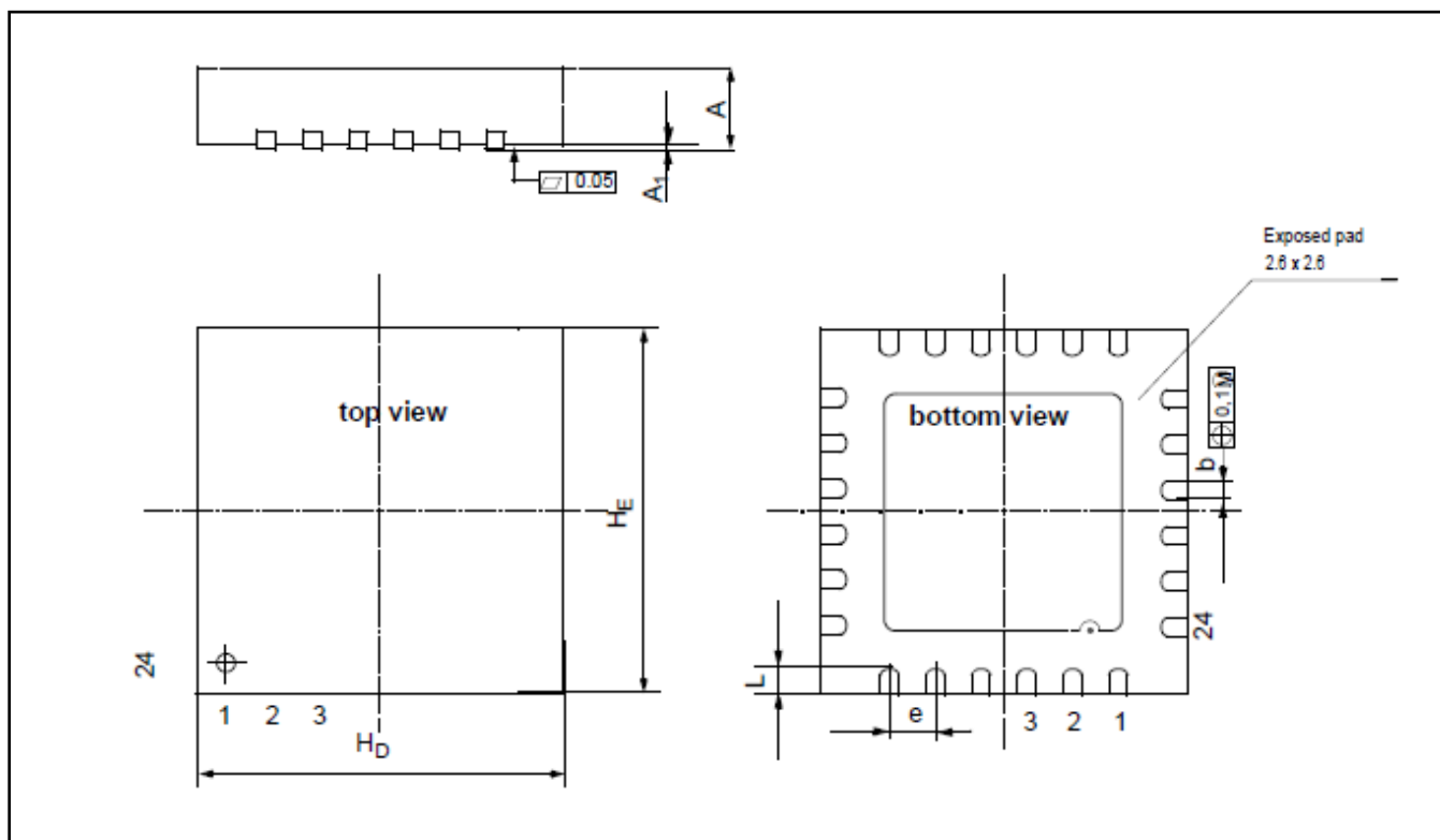
Figure 6.1 Package Drawing
