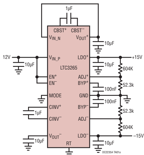
Low Noise \pm 15\text{V} Outputs from a Single 12V Input
