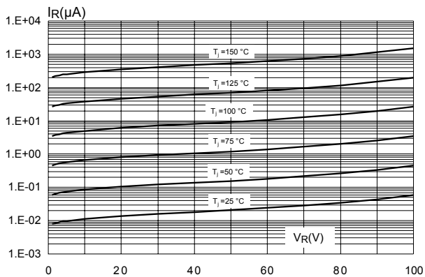
Figure 7. Reverse leakage current versus voltage applied (typical values)
