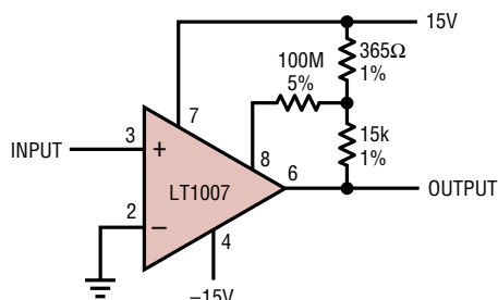
Microvolt Comparator with Hysteresis
