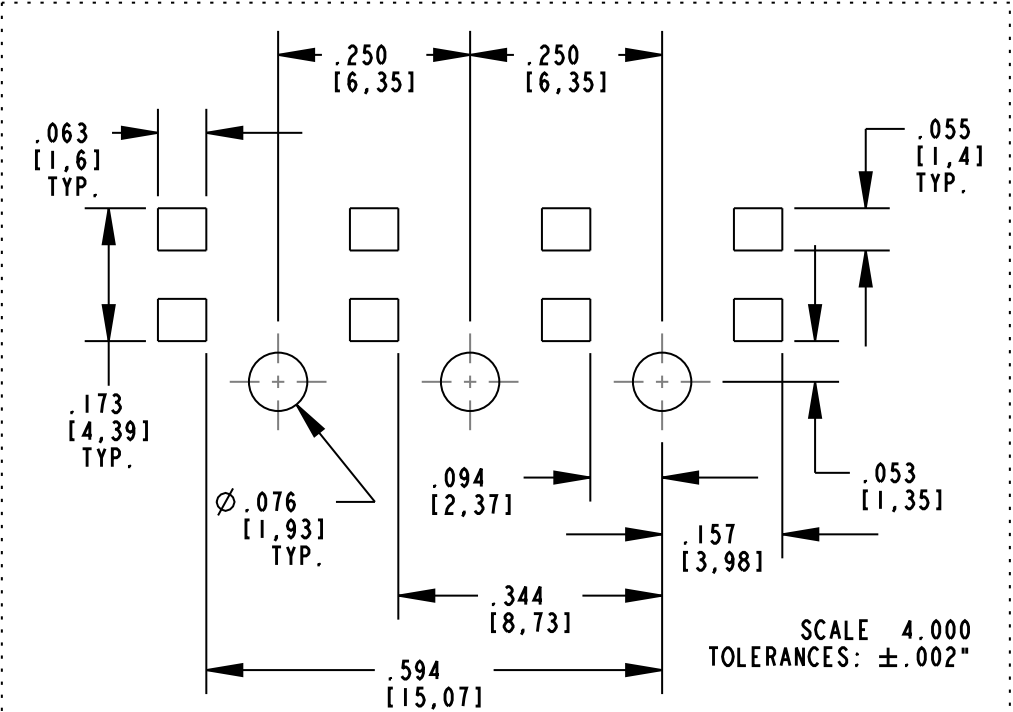
RECOMMENDED SOLDER PAD LAYOUT & HOLE PATTERN GAUGE
