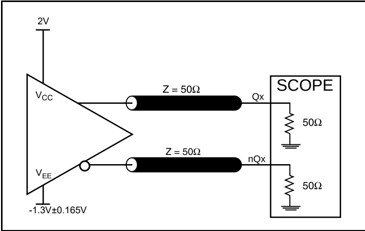
3.3V \pm 5\% LVPECL Output Load Test Circuit
