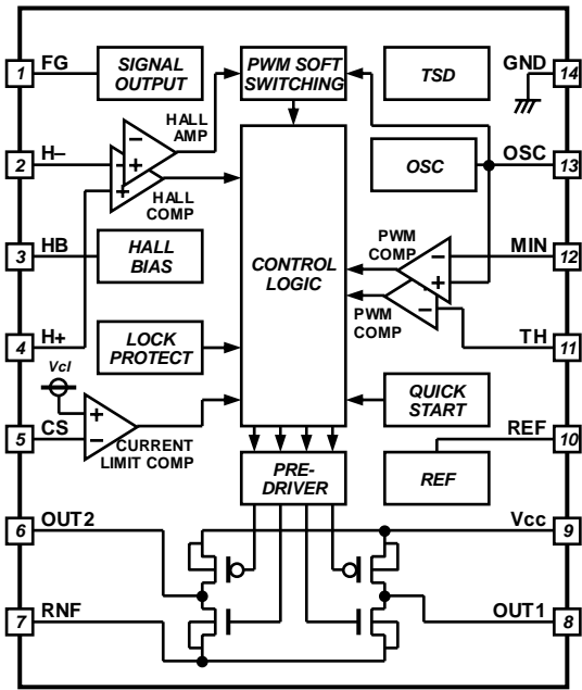
Fig.2 Block diagram
