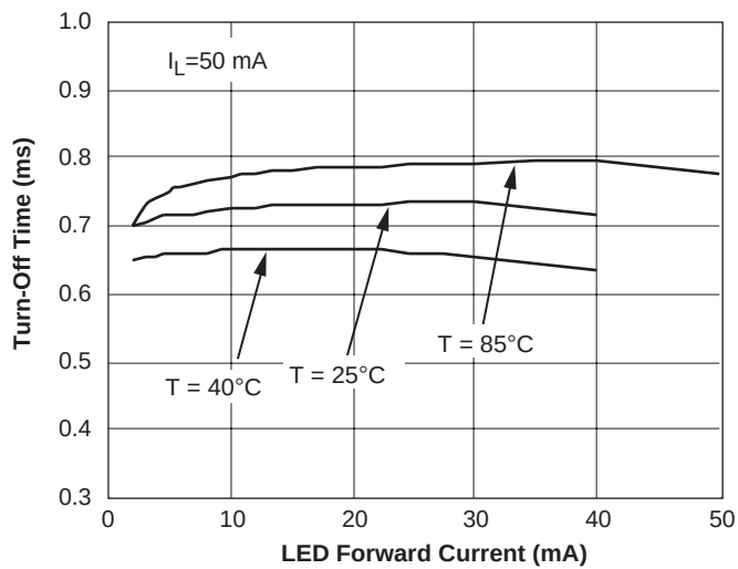
Figure 21. Turn-Off Time vs. LED Current
