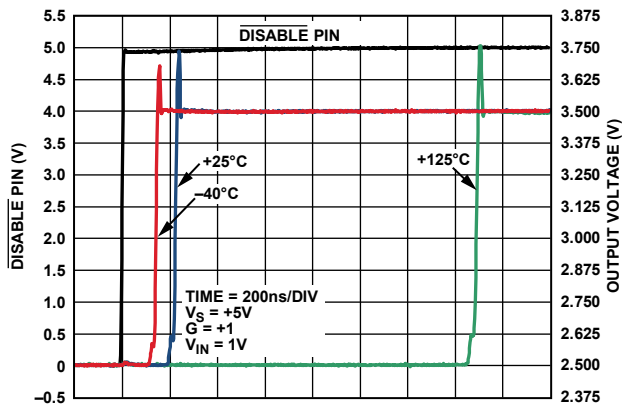
Figure 41. Turn-On Time vs. Temperature (ADA4897-1 and ADA4897-2)
