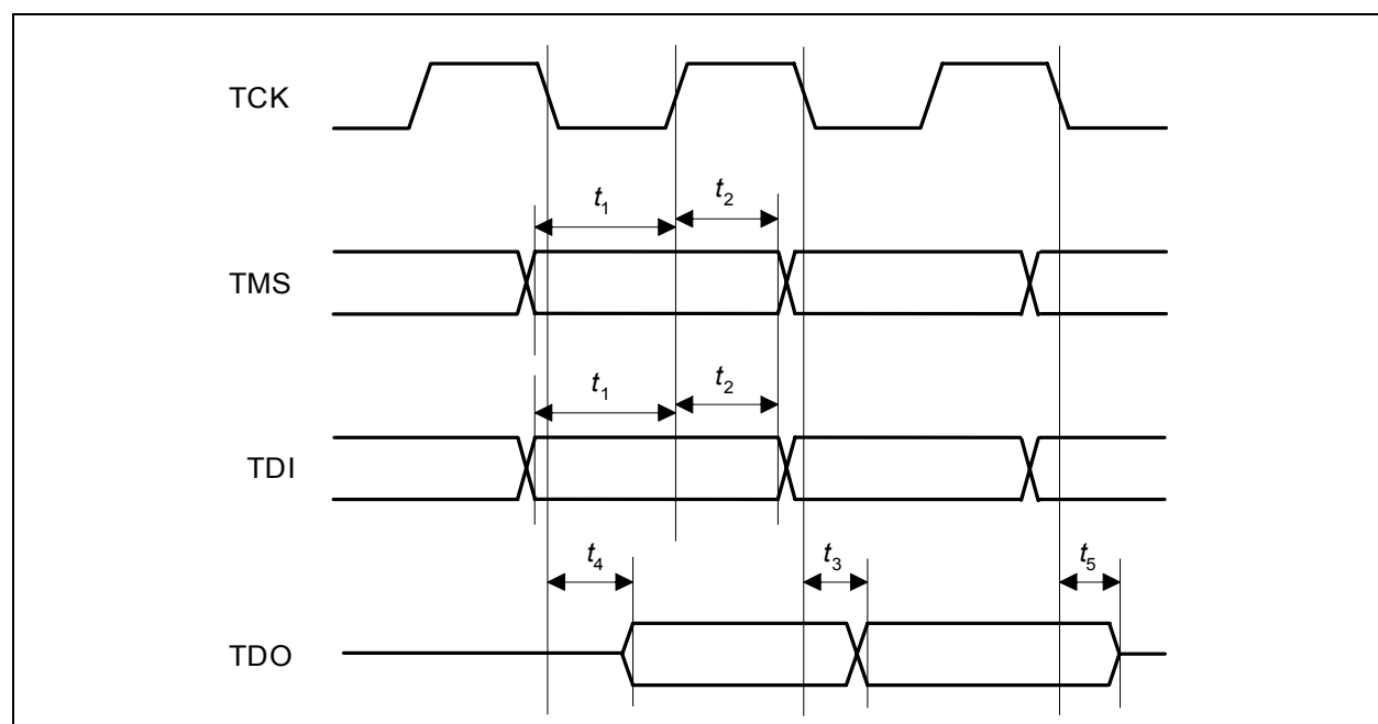
Figure 45 JTAG Timing
