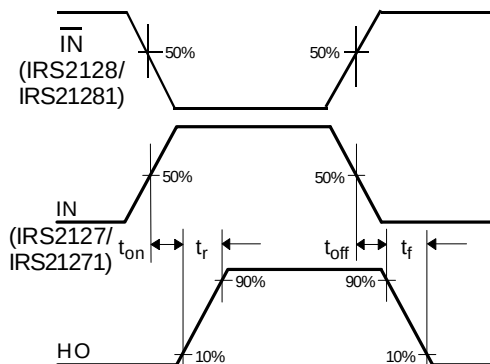
Figure 2. Switching Time Waveform Definition
