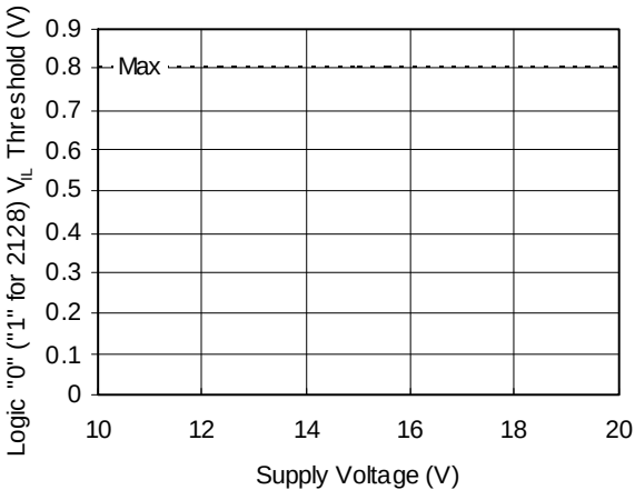
Figure 14B. Logic "0" ("1" for 2128) V_{IL} Threshold vs. Voltage
