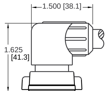
CABLE END ASSEMBLY 90° BOOT 0.445 [11.3] MAX. CABLE O.D.
