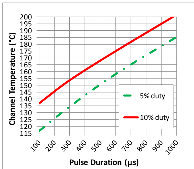
Max. Transient Channel Temp. vs. Pulse Width ( V_{DD} = 50 V)
