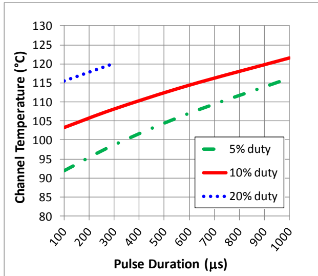
Max. Transient Channel Temp. vs. Pulse Width ( V_{DD} = 35 V)
