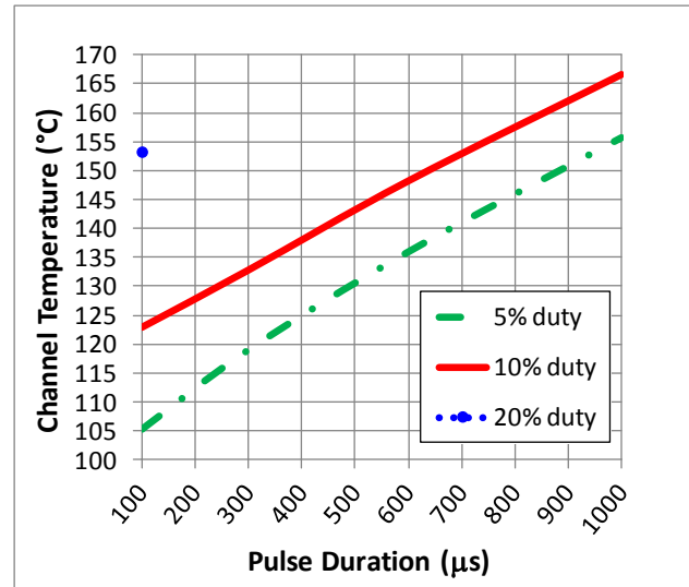
Max. Transient Channel Temp. vs. Pulse Width ( V_{DD} = 45 V)
