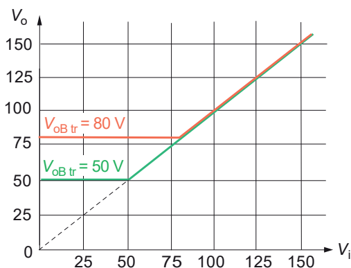
Fig. 1 V_o versus V_i depending on V_{oBr}
