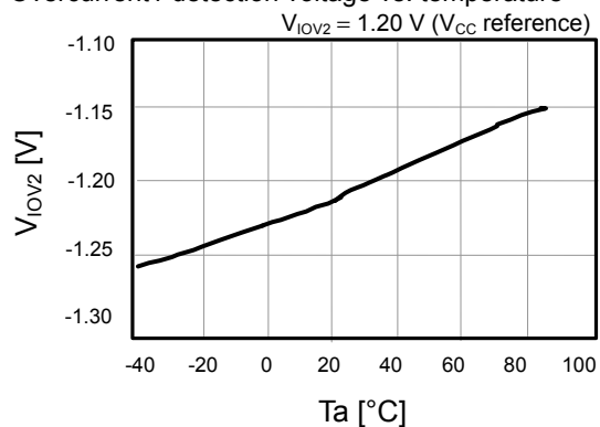
Overcurrent2 detection voltage vs. temperature
