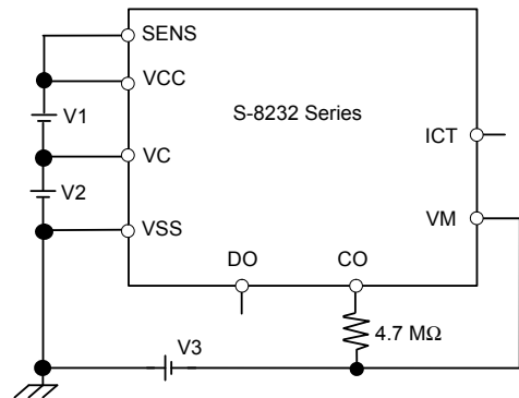
Test Circuit 6
