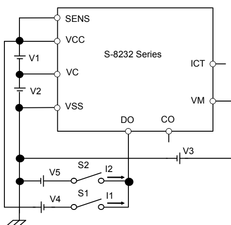
Test Circuit 3
