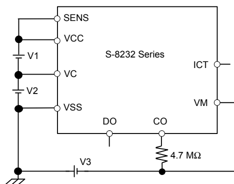
Test Circuit 6
