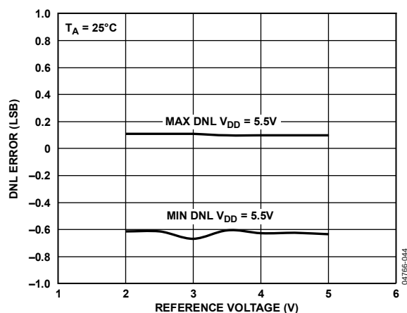
Figure 11. DNL Error vs. Reference Input Voltage
