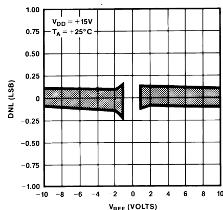
Figure 3. Differential Nonlinearity vs. V_{REF}
