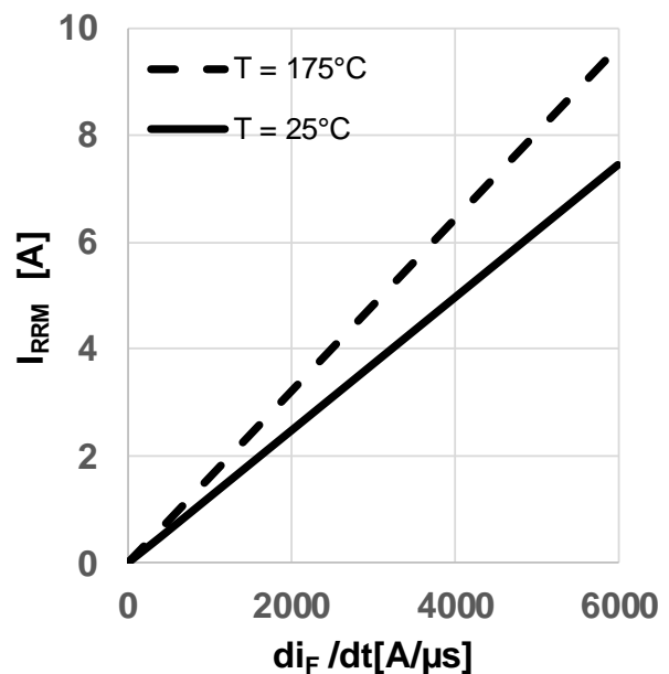
Figure 20 Typical reverse recovery current as a function of diode current slope (I_{rrm} = f(di_i/dt), V_{DD} = 800V, V_{GS} = 0V/18V, I_D = 6A, \text{ind. load, test circuit in Fig.E,} \text{body diode at } V_{GS} = 0V)
