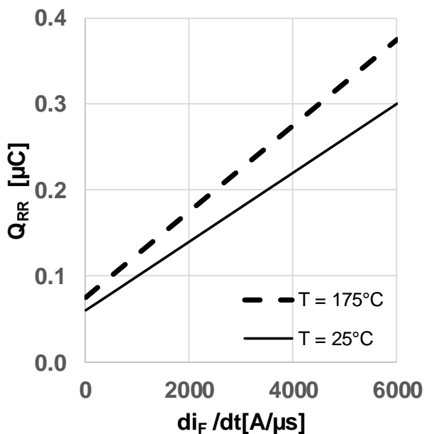
Figure 19 Typical reverse recovery charge as a function of diode current slope (Q_{rr} = f(di_i/dt), V_{DD} = 800V, V_{GS} = 0V/18V, I_D = 6A, \text{ind. load, test circuit in Fig.E, body} \text{diode at } V_{GS} = 0V)
