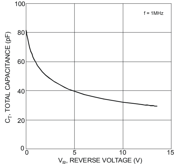
Figure 4 Typical Capacitance
