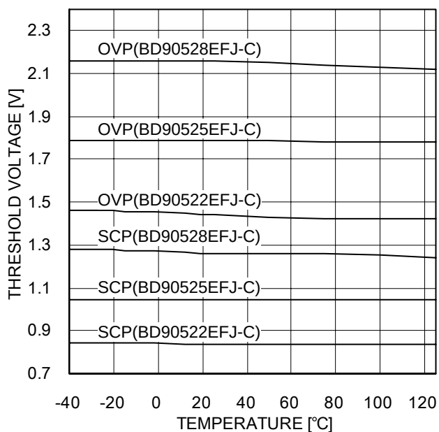
Figure 22. Output over/short detect voltage
