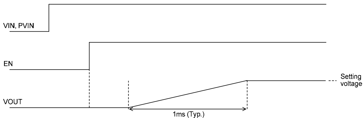
Figure 27. Start-up
