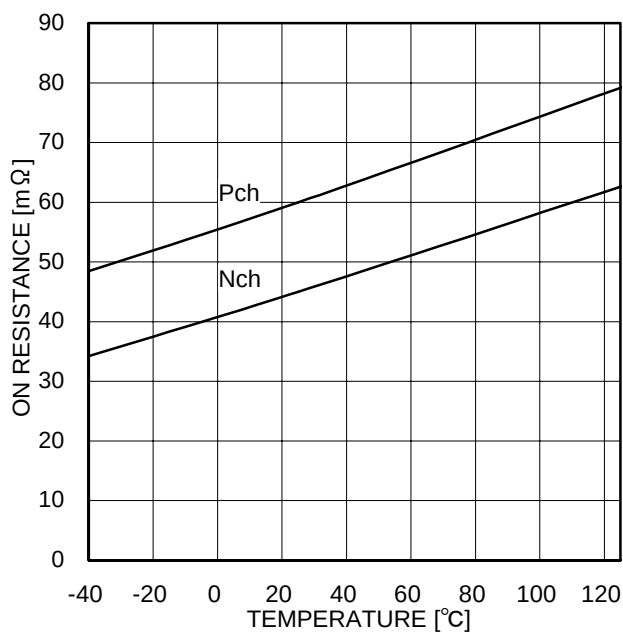
Figure 20. FET ON resistance
