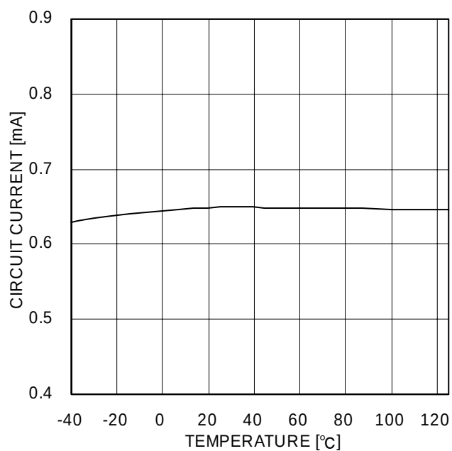
Figure 11. Circuit Current
