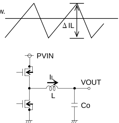
Figure 30. Ripple current
