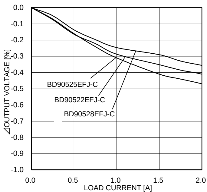
Figure 15. Load regulation
