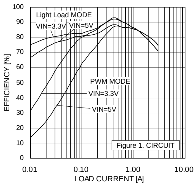
Figure 8. Efficiency(BD90525EFJ-C)
