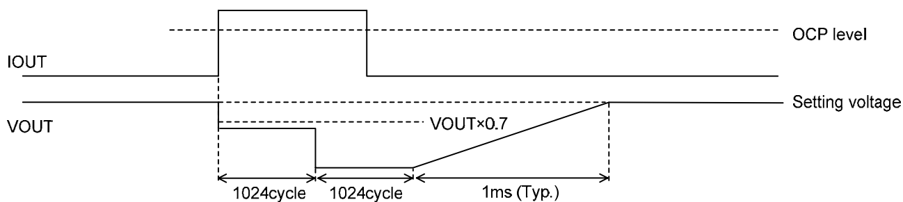
Figure 28. OCP
