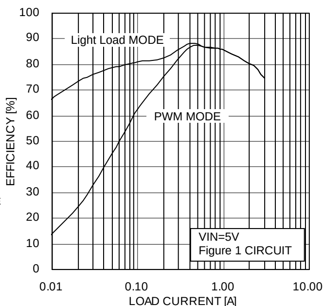
Figure 2. Efficiency (BD90525EFJ-C)
