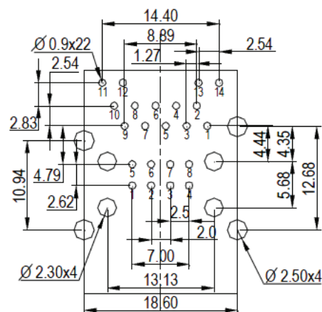
Recommended PCB Layout Component Side Shown
