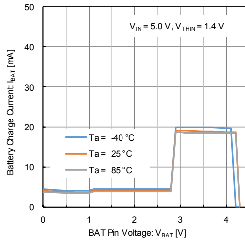
(11) Battery Charge Current vs. BAT Pin Voltage ( R_{ISET} = 20 k \Omega , Cold Operation)
