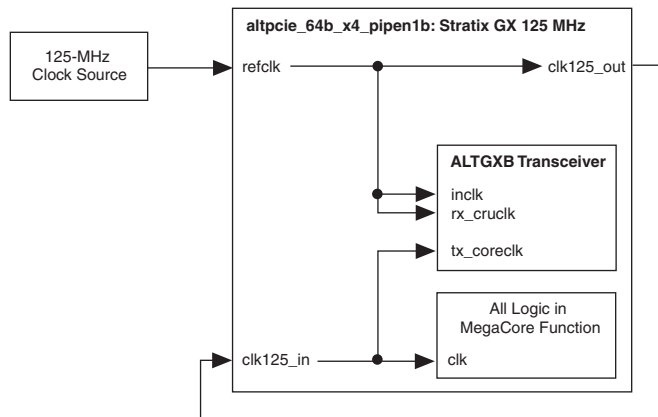
Figure 3–31. Stratix GX PHY, 125 MHz Reference Clock Configuration (1)
