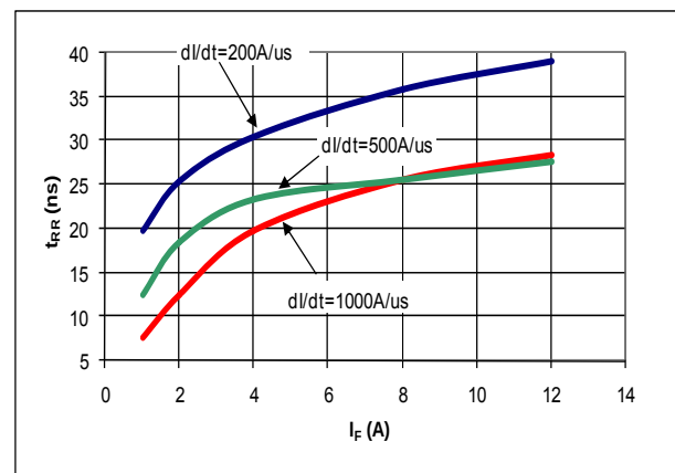
Figure 6. Typical t_{RR} vs I_F at T_J = 125\text{ }^{\circ}
