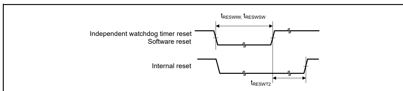
Figure 5.31 Reset Input Timing (2)
