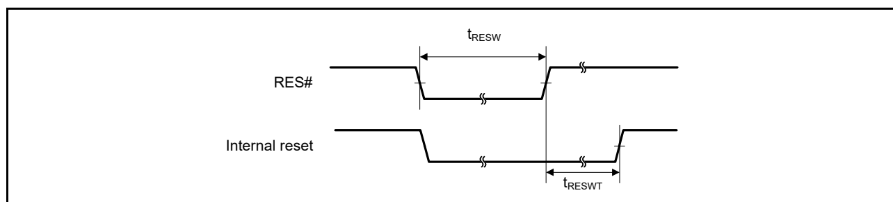
Figure 5.30 Reset Input Timing (1)
