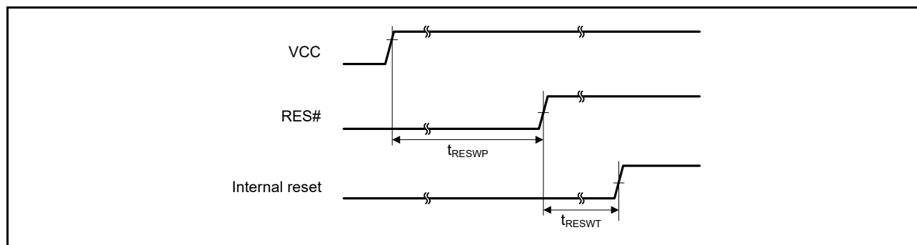
Figure 5.29 Reset Input Timing at Power-On
