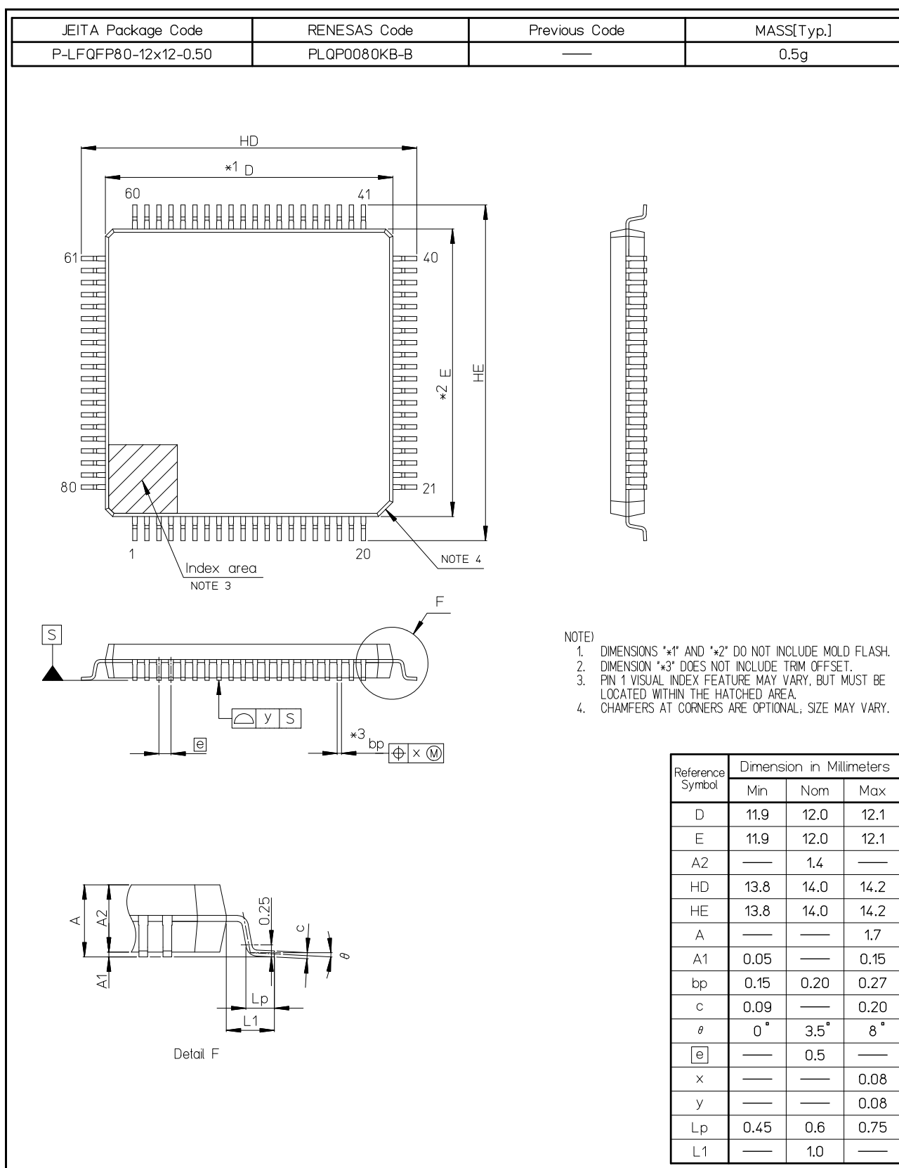
Figure C 80-Pin LFQFP (PLQP0080KB-B)
