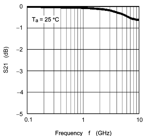
Fig. 9.5 S_{21} - f
