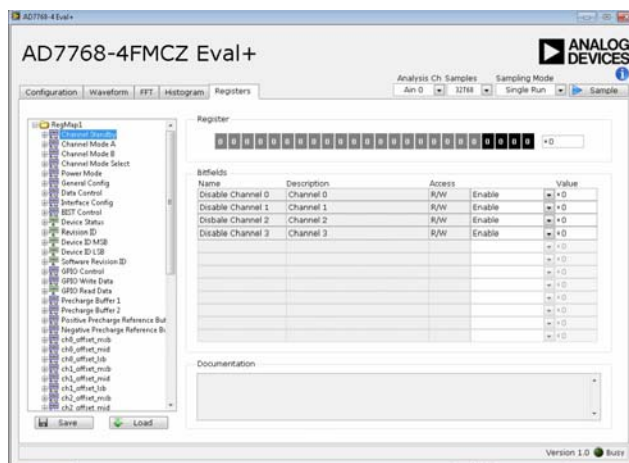
Figure 21. Registers Tab
