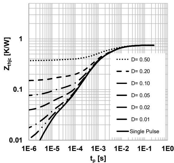
Figure 7. Max. transient thermal impedance, Z_{th,j-c}=f(t_P) , parameter: D=t_P/T
