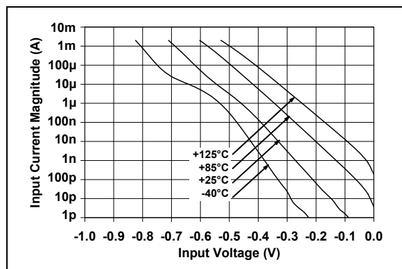
FIGURE 2-33: Input Current vs. Input Voltage (Below V_{SS} ).
