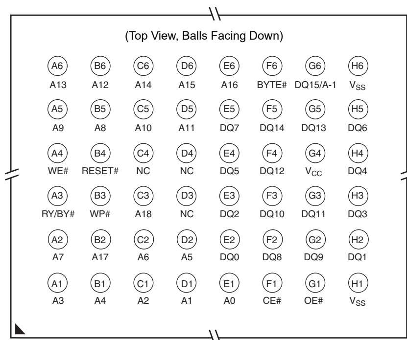
Figure 2. 48-ball Fine-pitch BGA (VBK048)
