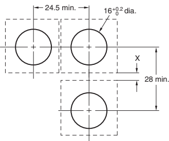
Panel Cutout (Top View)
